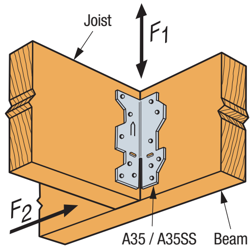
SIMPSON Strong-Tie® A35/A35SS Joist-to-Beam Installation
