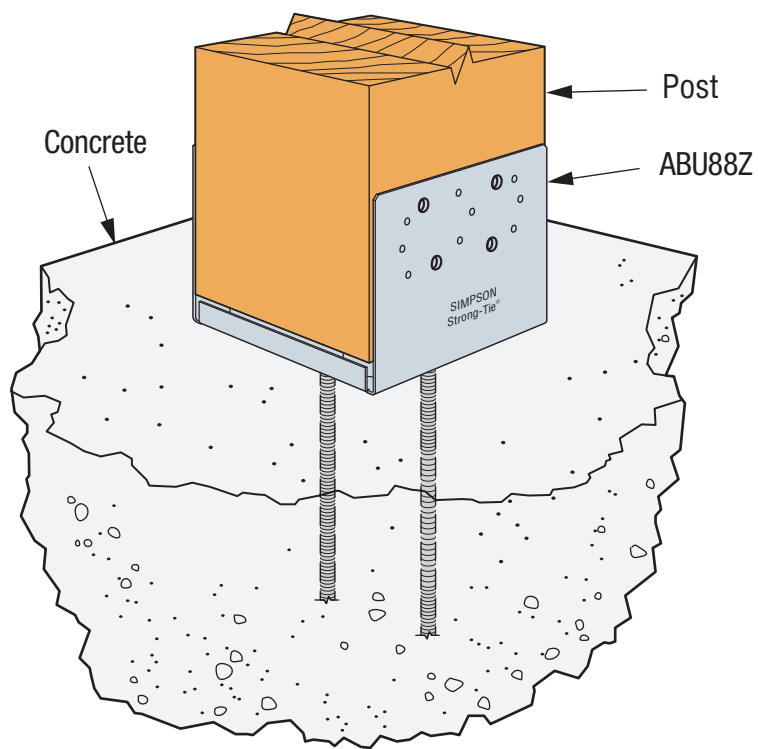
SIMPSON Strong-Tie® ABU88Z Post Base Installation
