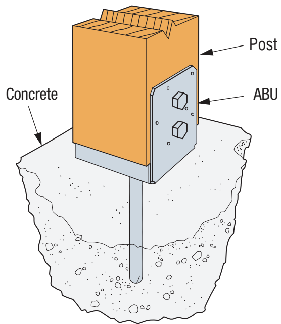
SIMPSON Strong-Tie® ABU Post Base Installation
