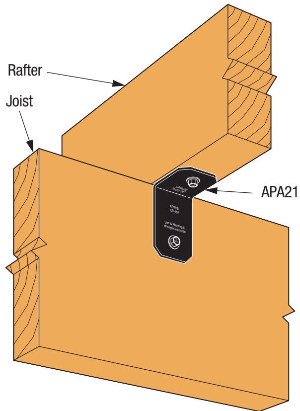
SIMPSON Strong-Tie® APA21 Joist-to-Rafter Installation
