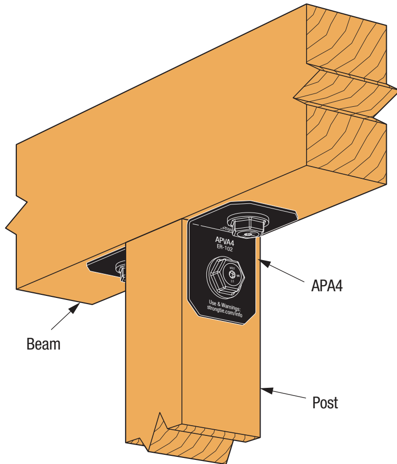
SIMPSON Strong-Tie® APA4 Post-to-Beam Installation
