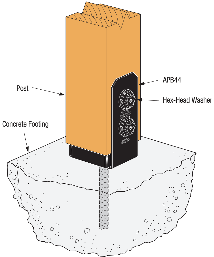
SIMPSON Strong-Tie® APB44 Post Base Connection
