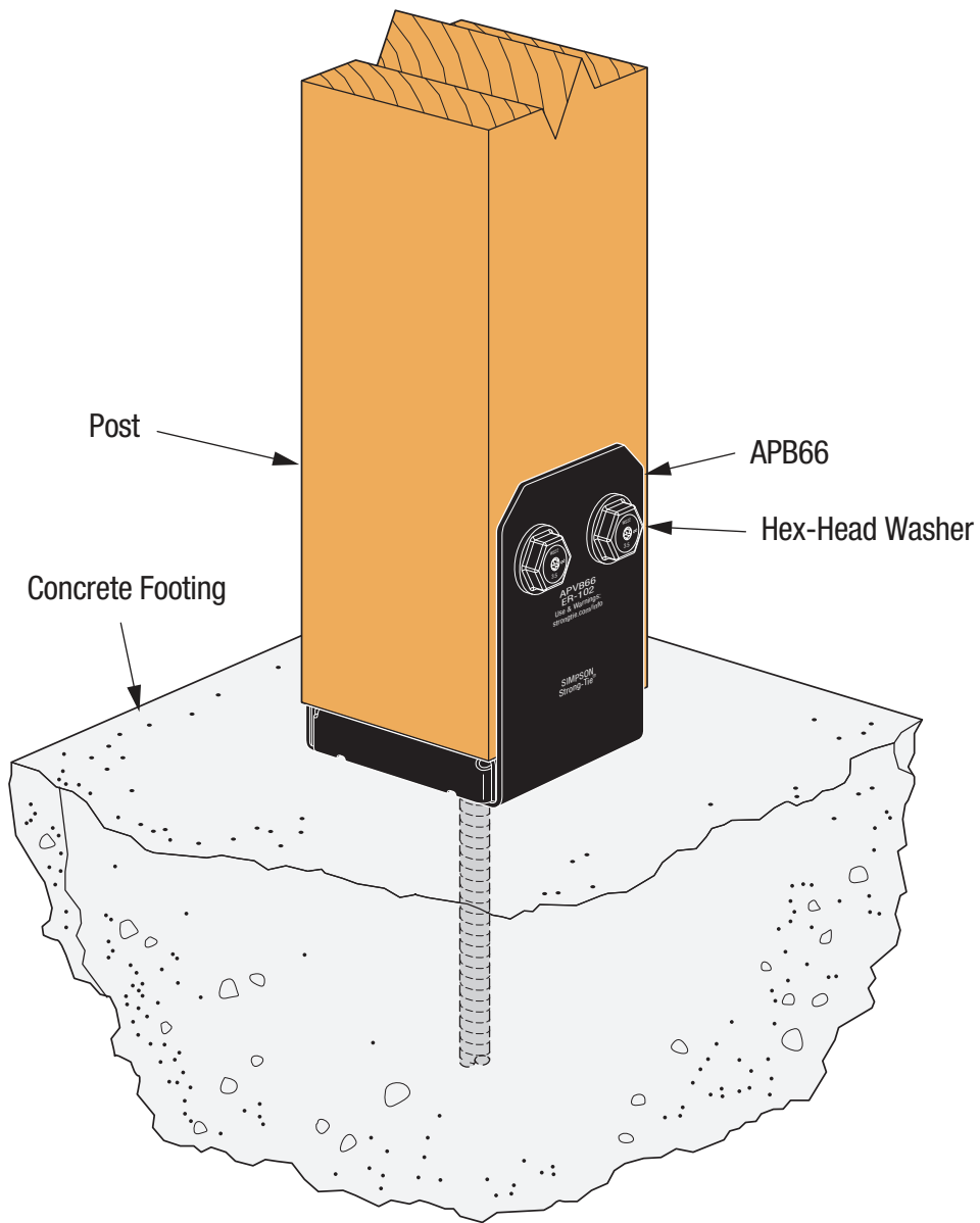
SIMPSON Strong-Tie® APB66 Post Base Connection
