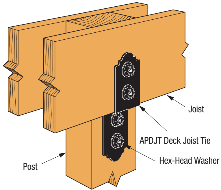
SIMPSON Strong-Tie® APDJT Joist-to-Post Connection
