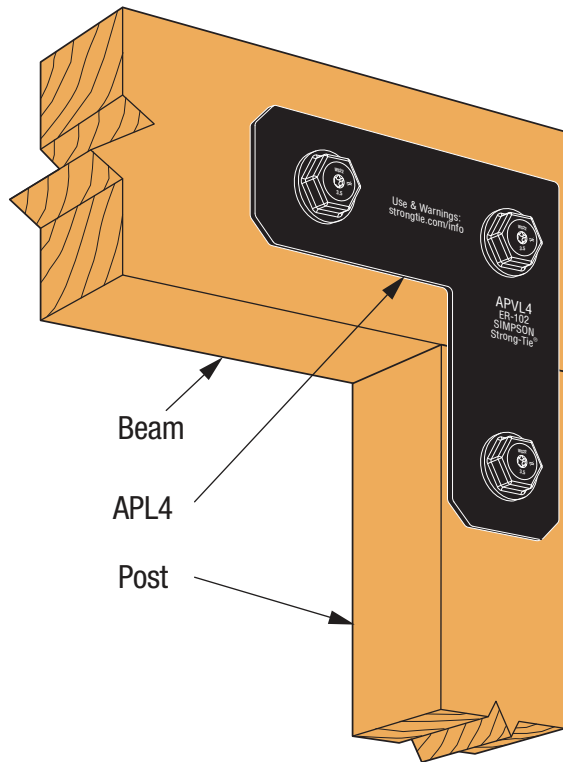
SIMPSON Strong-Tie® APL4 Post-to-Beam Corner Installation
