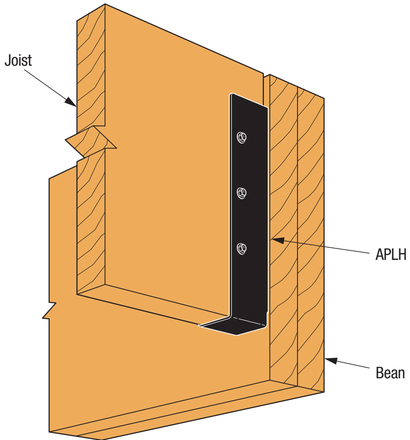
SIMPSON Strong-Tie® APLH Joist-to-Beam Installation
