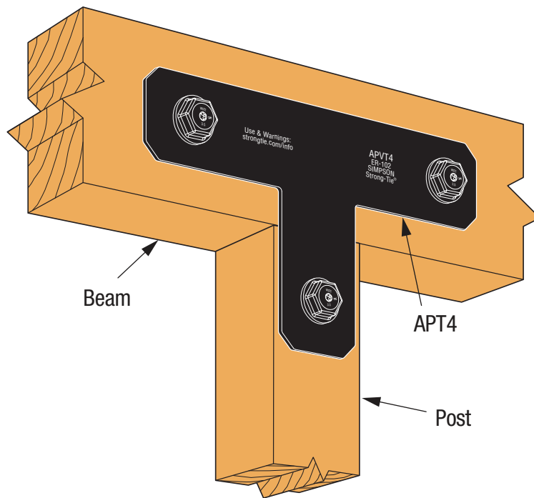
SIMPSON Strong-Tie® APT4 Post-to-Beam Installation
