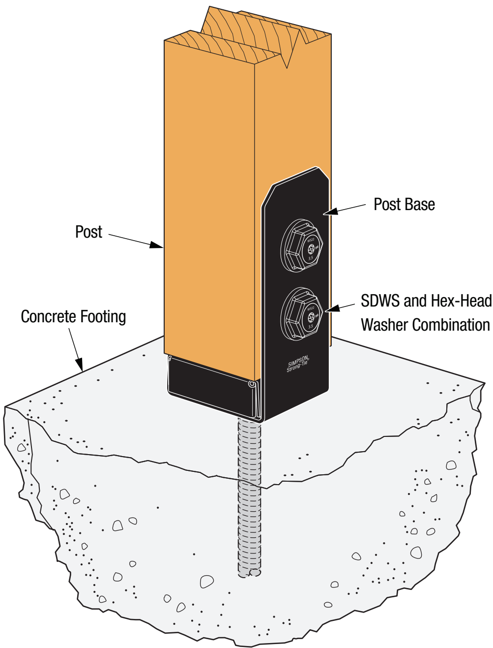
SIMPSON Strong-Tie® APVB90 Post Base Connection
