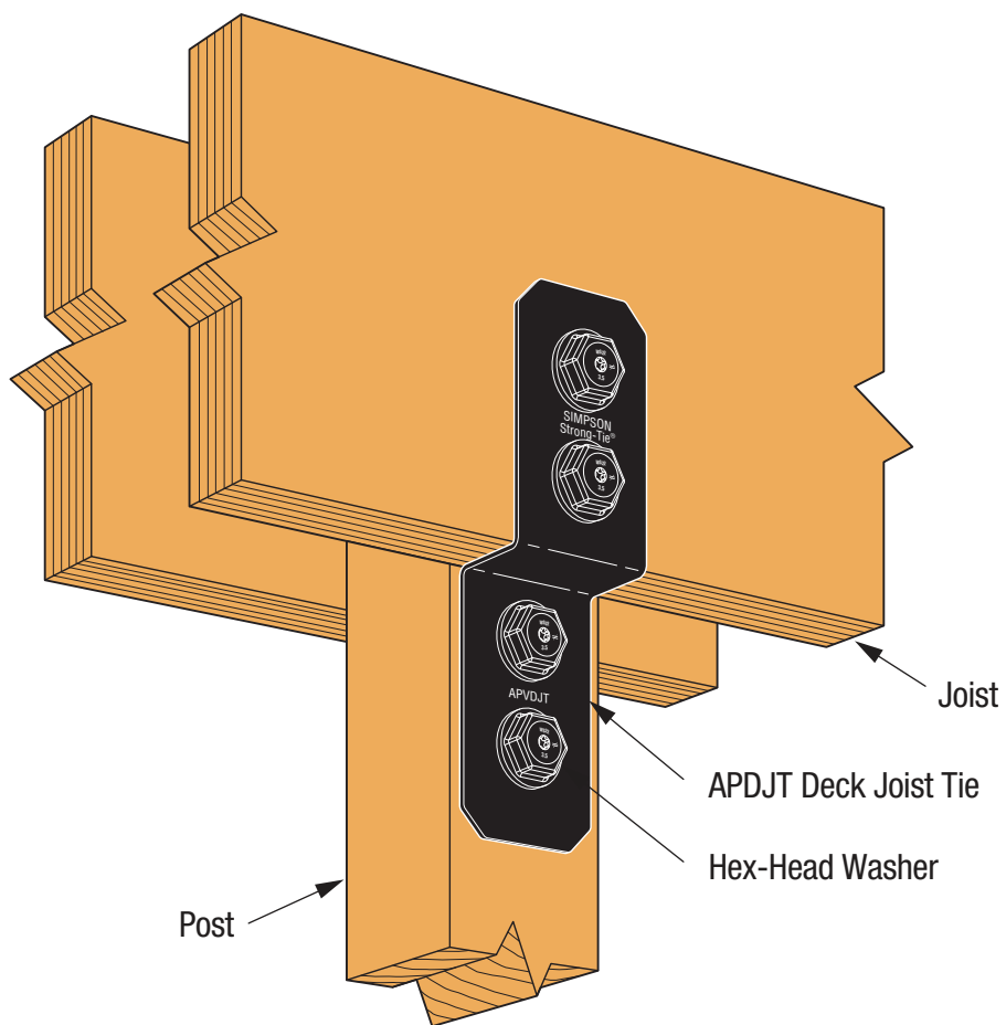
SIMPSON Strong-Tie® APDJT Joist-to-Post Connection
