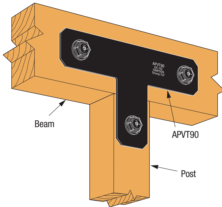
SIMPSON Strong-Tie® APVT90 Post-to-Beam Installation
