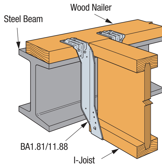
SIMPSON Strong-Tie® BA Top Fix I-Joist Installation on Wood Nailer
