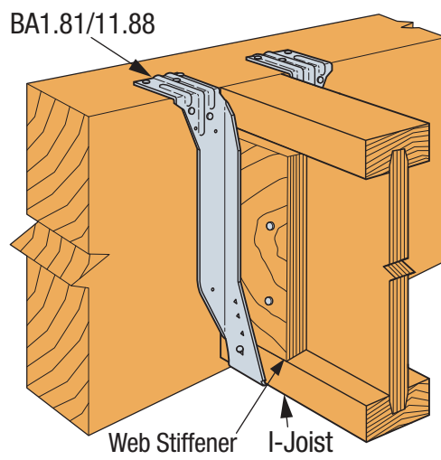
SIMPSON Strong-Tie® BA Top Fix I-Joist Installation with Web Stiffeners
