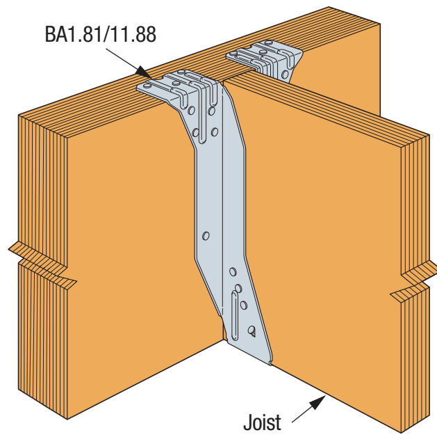
SIMPSON Strong-Tie® BA Top Fix Joist Installation
