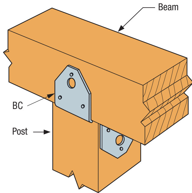
SIMPSON Strong-Tie® BC Post Cap Installation
