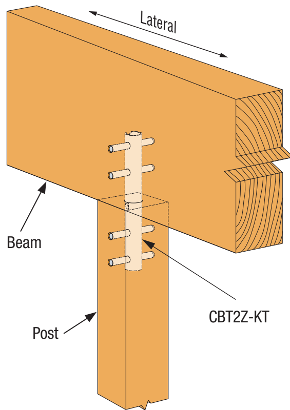
SIMPSON Strong-Tie® CBT2Z Beam-to-Post Installation
