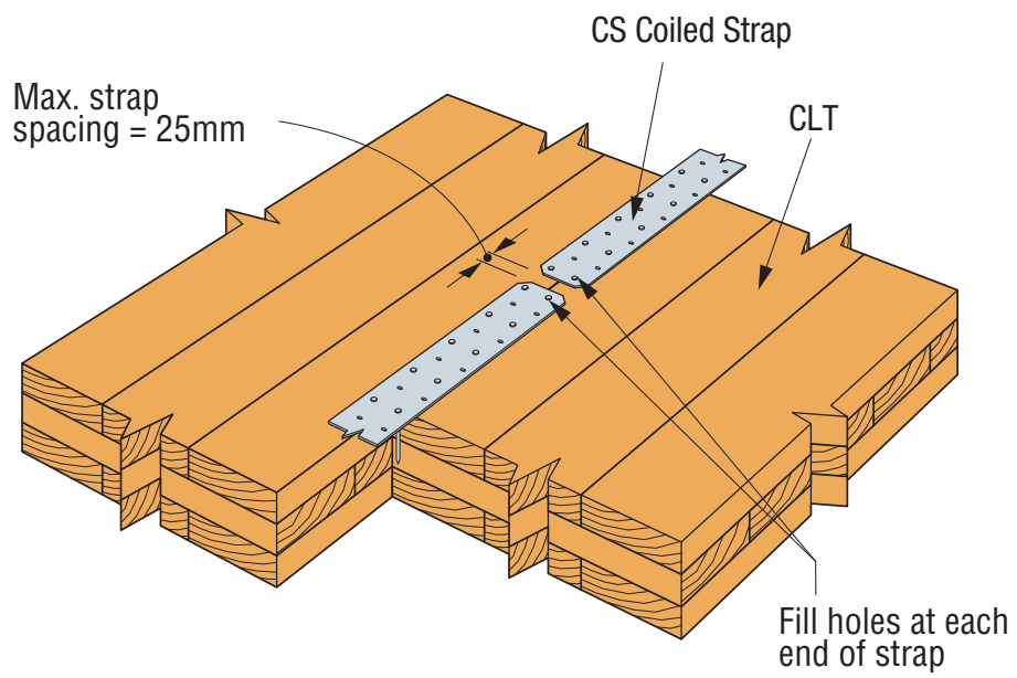
SIMPSON Strong-Tie® CS Installation - CLT Panel
