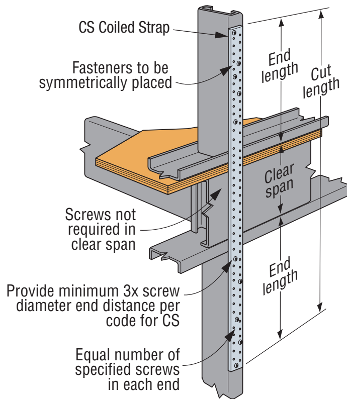
SIMPSON Strong-Tie® CS Floor-to-Floor Tie Installation - Steel Frame
