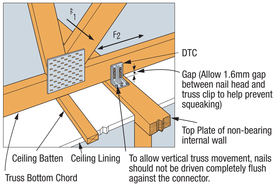
SIMPSON Strong-Tie® DTC Installation
