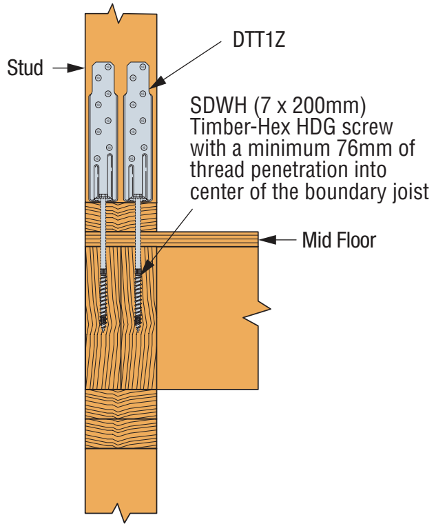
SIMPSON Strong-Tie® DTT1Z Mid Floor Wall Bracing
