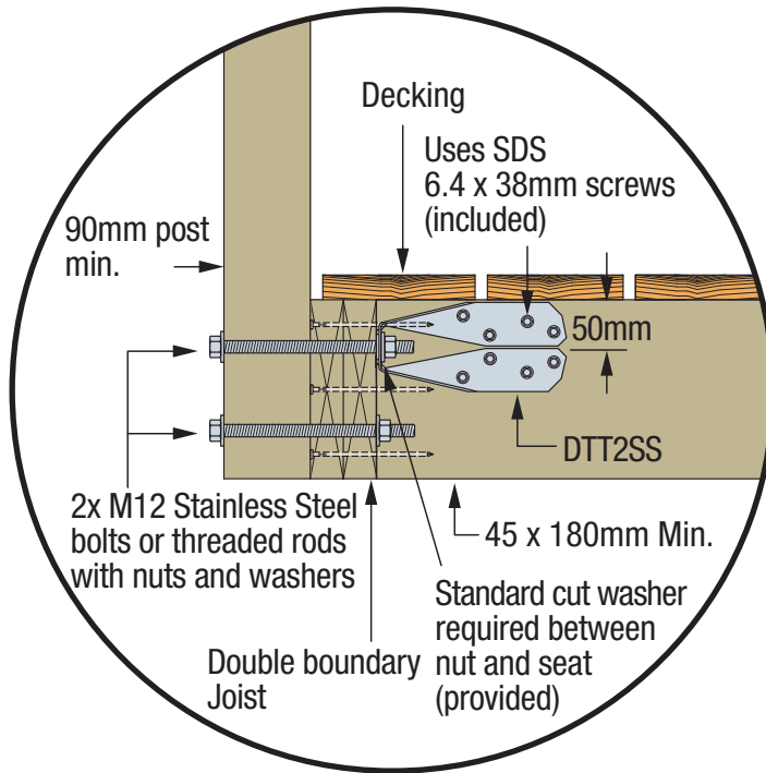
SIMPSON Strong-Tie® DTT2SS Deck Post Connection
