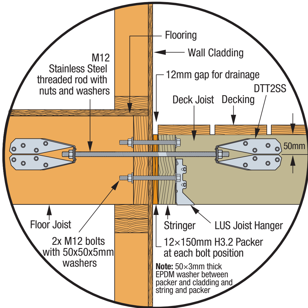
SIMPSON Strong-Tie® DTT2SS Deck-to-House Lateral Load Connection
