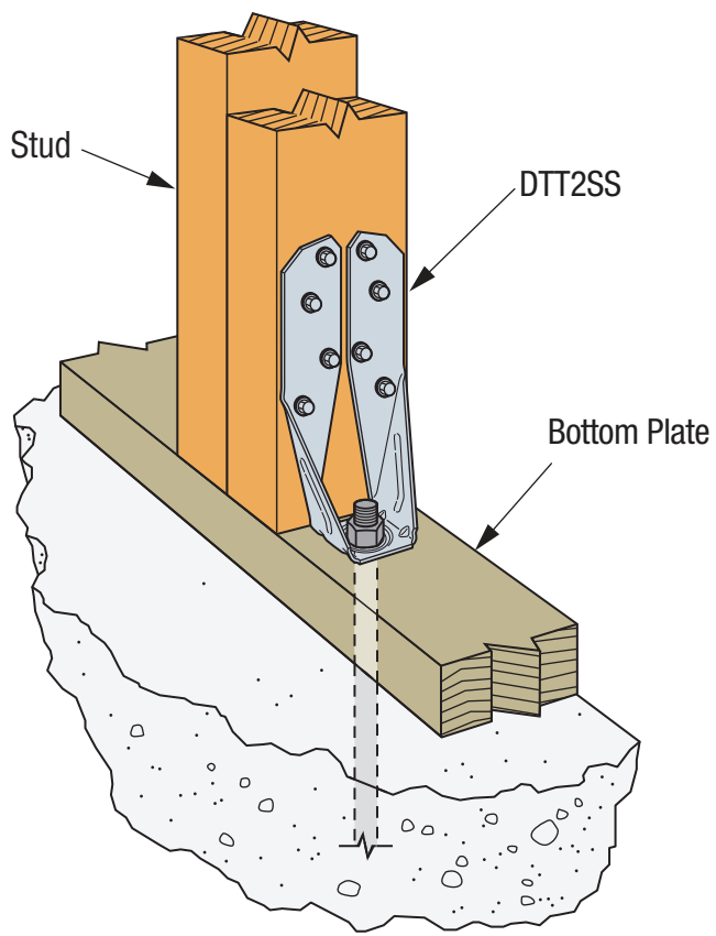
SIMPSON Strong-Tie® DTT2SS Holdown Installation
