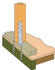
DTT1Z Holddown
