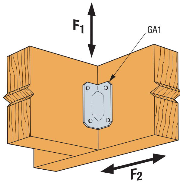
SIMPSON Strong-Tie® GA1 Installation
