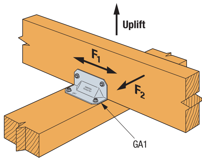
SIMPSON Strong-Tie® GA1 Installation
