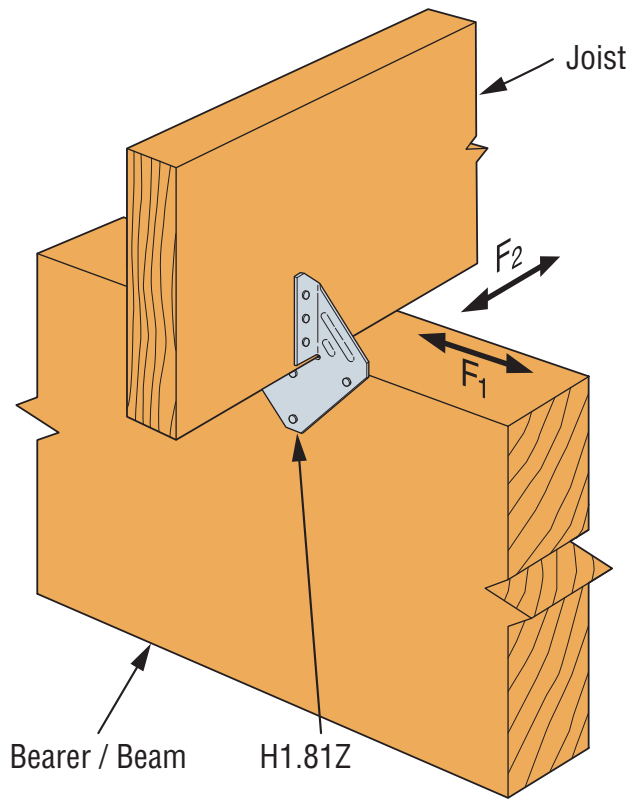
SIMPSON Strong-Tie® H1.81Z Bearer/Beam-to-Joist Tie Down
