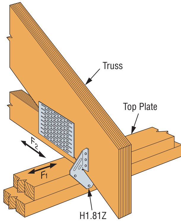
SIMPSON Strong-Tie® H1.81Z Truss-to-Top Plate Tie Down
