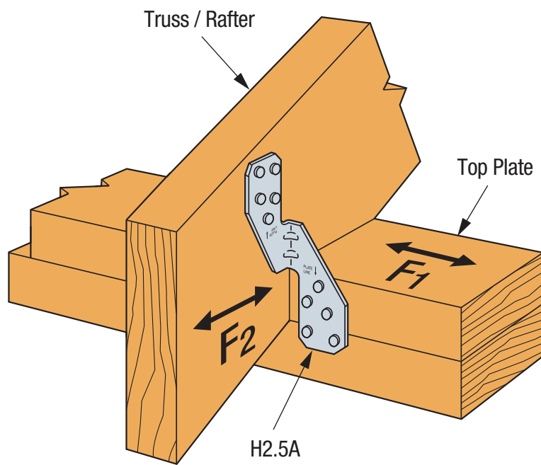
SIMPSON Strong-Tie® H2.5A Truss/Rafter-to-Top Plate Tie Down
