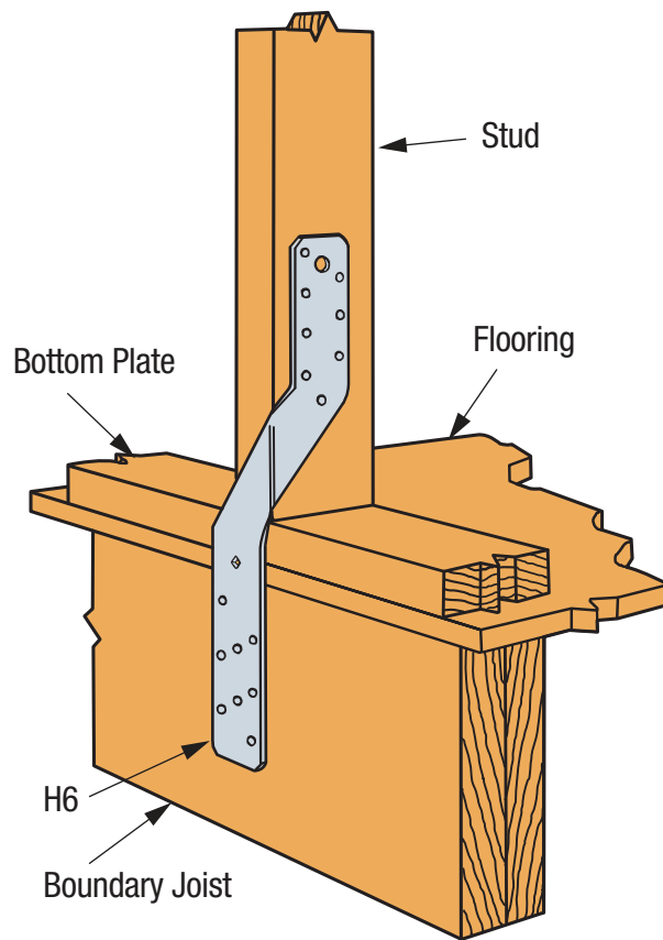
SIMPSON Strong-Tie® H6 Mid Floor Stud-to-Boundary Joist Tie Down
