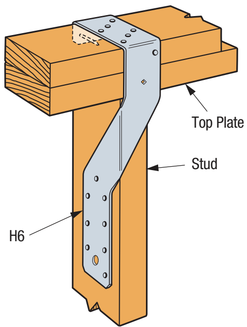
SIMPSON Strong-Tie® H6 Stud-to-Top Plate Tie Down
