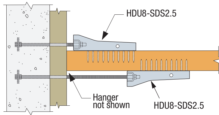
SIMPSON Strong-Tie® HDU8-SDS2.5 Lateral Load Connection
