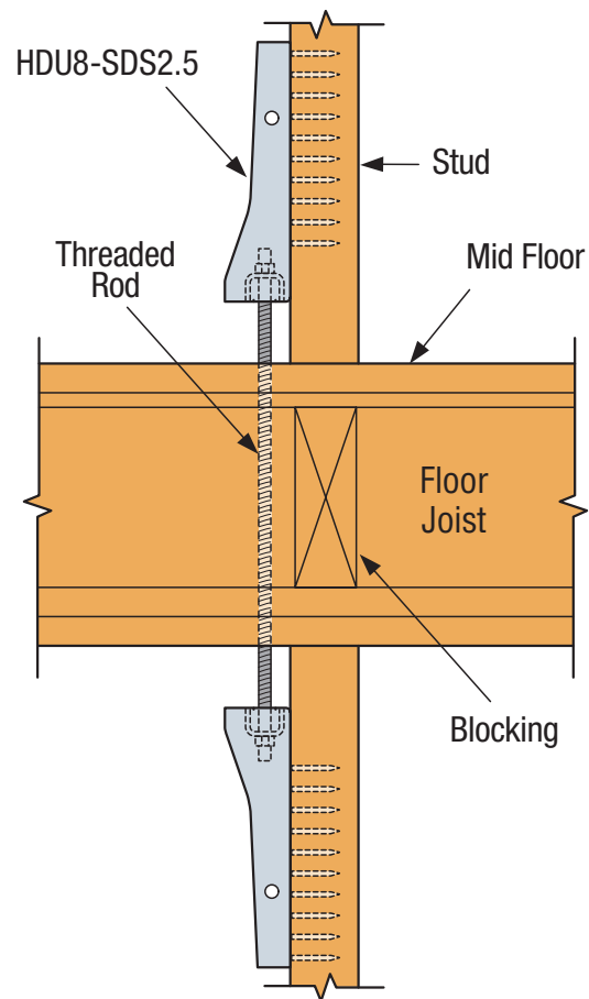
SIMPSON Strong-Tie® HDU8-SDS2.5 Mid Floor Holdown Installation
