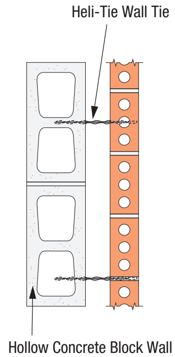
SIMPSON Strong-Tie® Heli-Tie Wall Tie Installation
