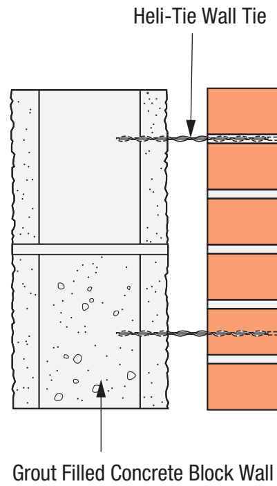
SIMPSON Strong-Tie® Heli-Tie Wall Tie Installation
