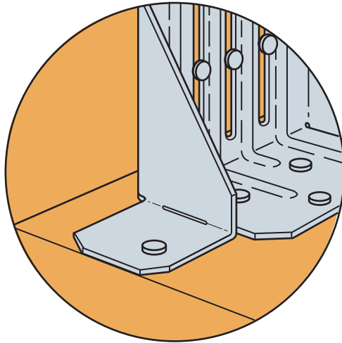
SIMPSON Strong-Tie® HTC Installation on a 140 x 45mm or Larger Plate
