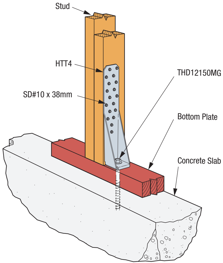
SIMPSON Strong-Tie® HTT4-KTM Bracewall Holdown Installation
