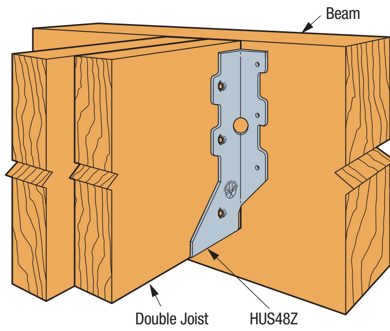
SIMPSON Strong-Tie® HUS48Z Double Joist Installation
