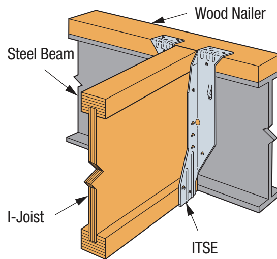
SIMPSON Strong-Tie® ITSE Top Fix I-Joist Installation on Wood Nailer
