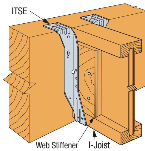
SIMPSON Strong-Tie® ITSE Top Fix I-Joist Installation with Web Stiffeners
