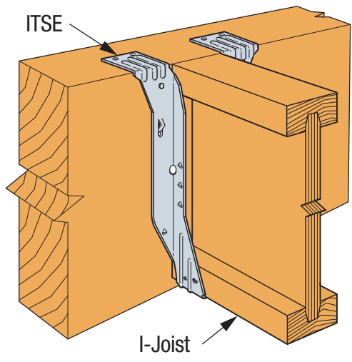
SIMPSON Strong-Tie® ITSE Top Fix I-Joist Installation
