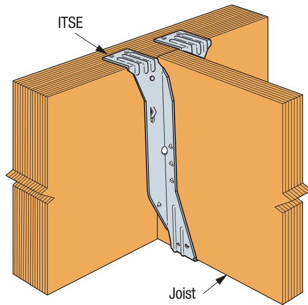
SIMPSON Strong-Tie® ITSE Top Fix Joist Installation
