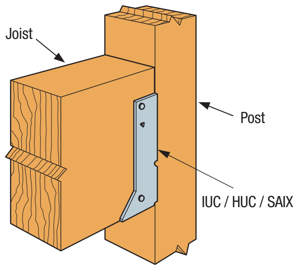
SIMPSON Strong-Tie® IUC/HUC/SAIX Installation on a Post
