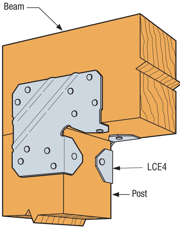
SIMPSON Strong-Tie® LCE4 Installation
