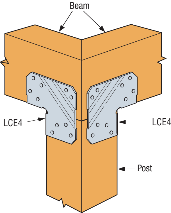
SIMPSON Strong-Tie® LCE4 Corner Installation
