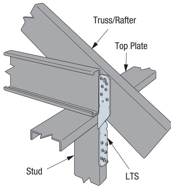
SIMPSON Strong-Tie® LTS Steel Frame Installation
