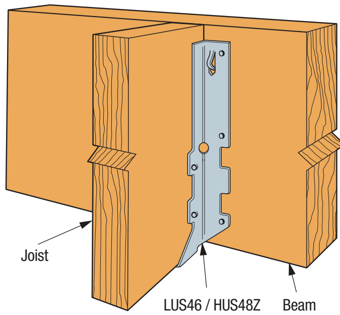
SIMPSON Strong-Tie® LUS46 / HUS48Z Installation
