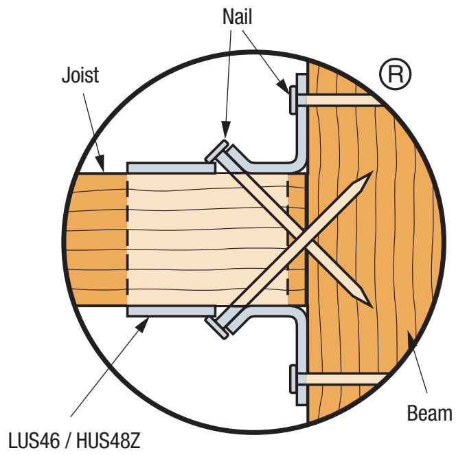
SIMPSON Strong-Tie® LUS46 / HUS48Z Double Shear Nailing Installation
